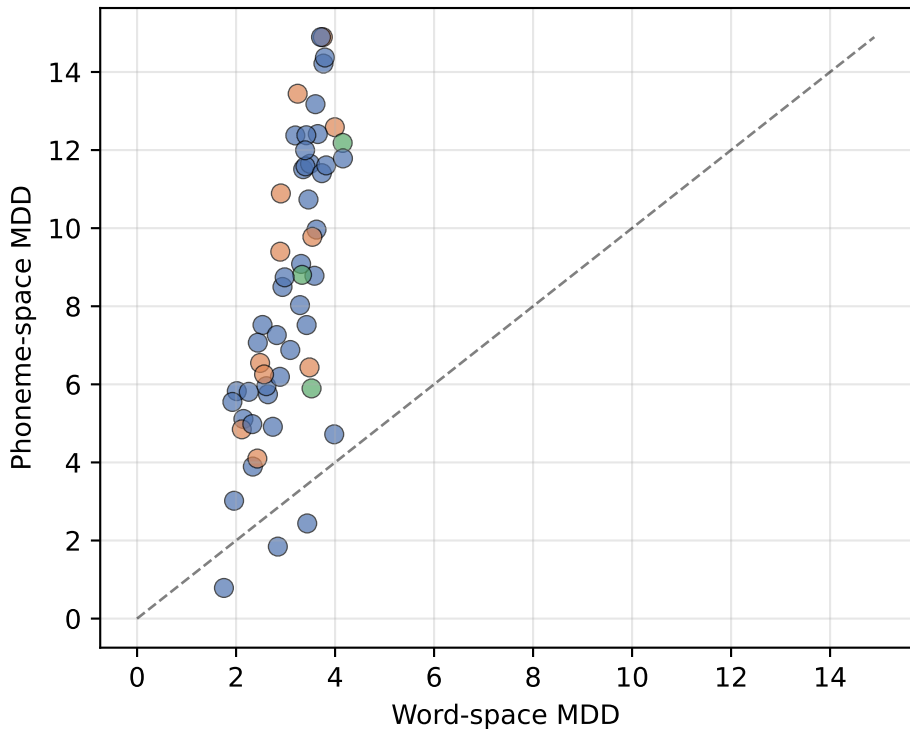
Word-space vs Phoneme-space Dependency Distance (n=55)
