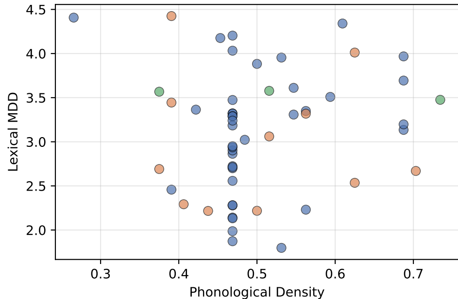
Lexical Dependencies
