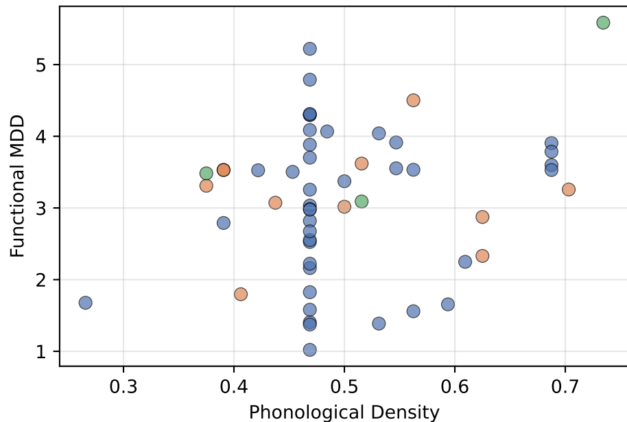
Functional Dependencies
