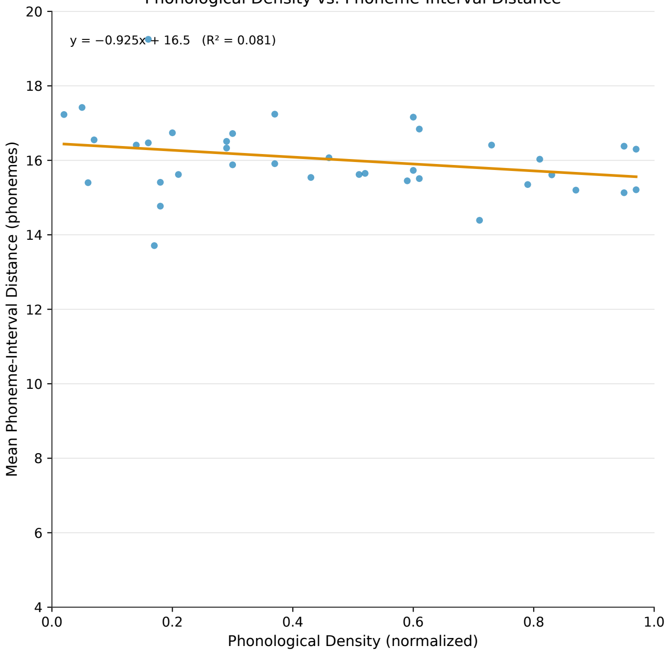
Phonological Density vs. Phoneme-Interval Distance
