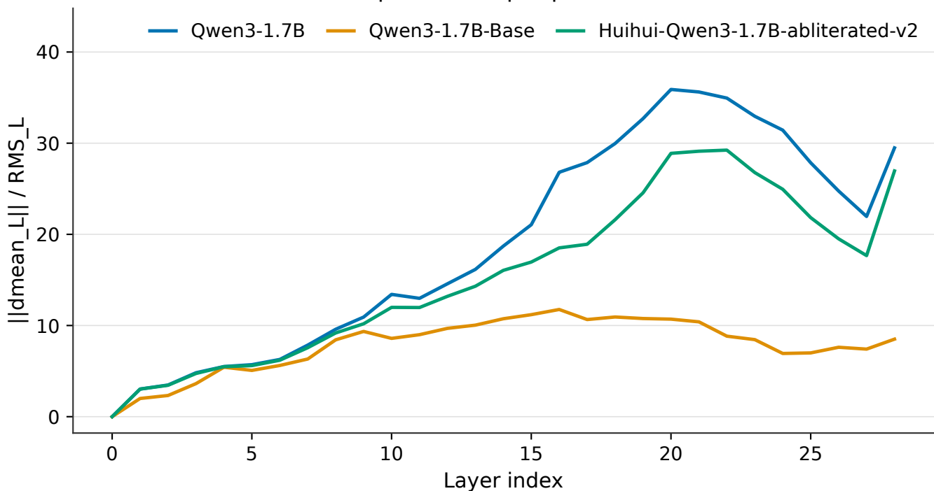
RMS-normalised separation depth profile (Qwen3-1.7B triad)
