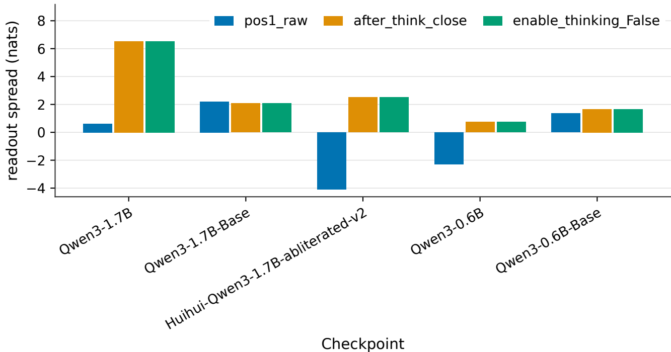
Gate G2: the thinking block moves the refusal readout
