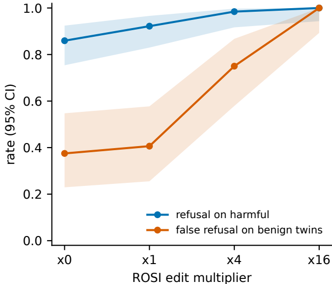
components, n=64 / 32 items 20-token greedy continuations
