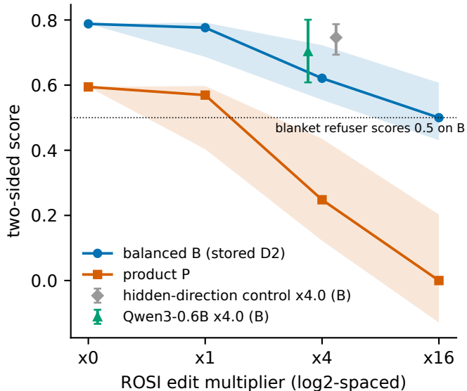
Qwen2.5-0.5B-Instruct dose response n=64 harmful + 32 twin items
