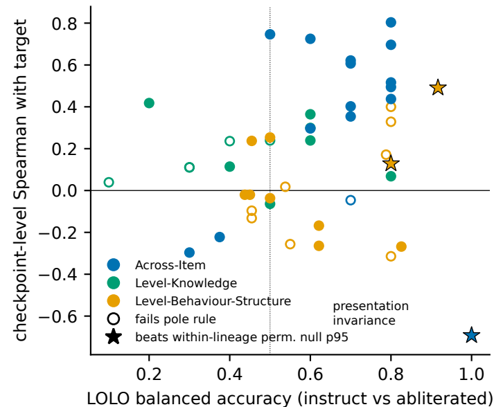
balanced target B 46 metrics, n=7-15 ckpts each
