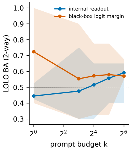
LOLO BA (stored, 200 item draws)
