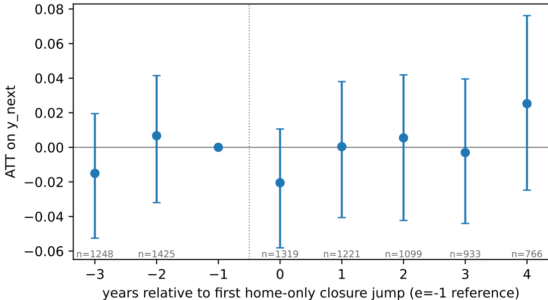
OLD_HELDOUT - primary_never (Sun-Abraham IW, 300 boots)
