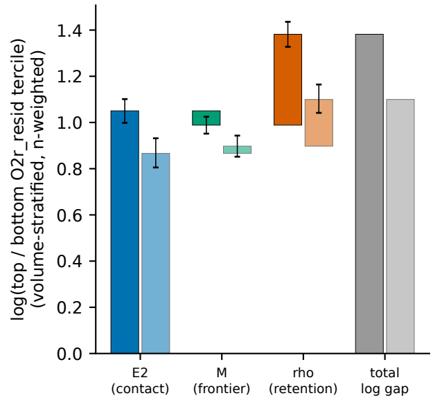
DEV (CS/Eng/BGM/Med)
