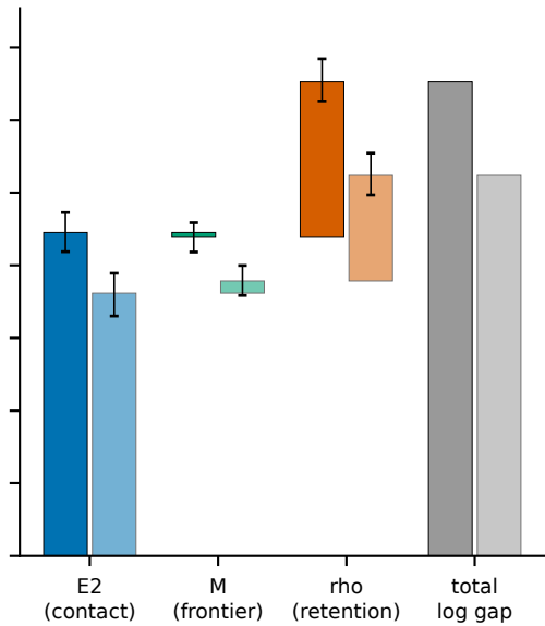
Cohort 2010-14 pooled
