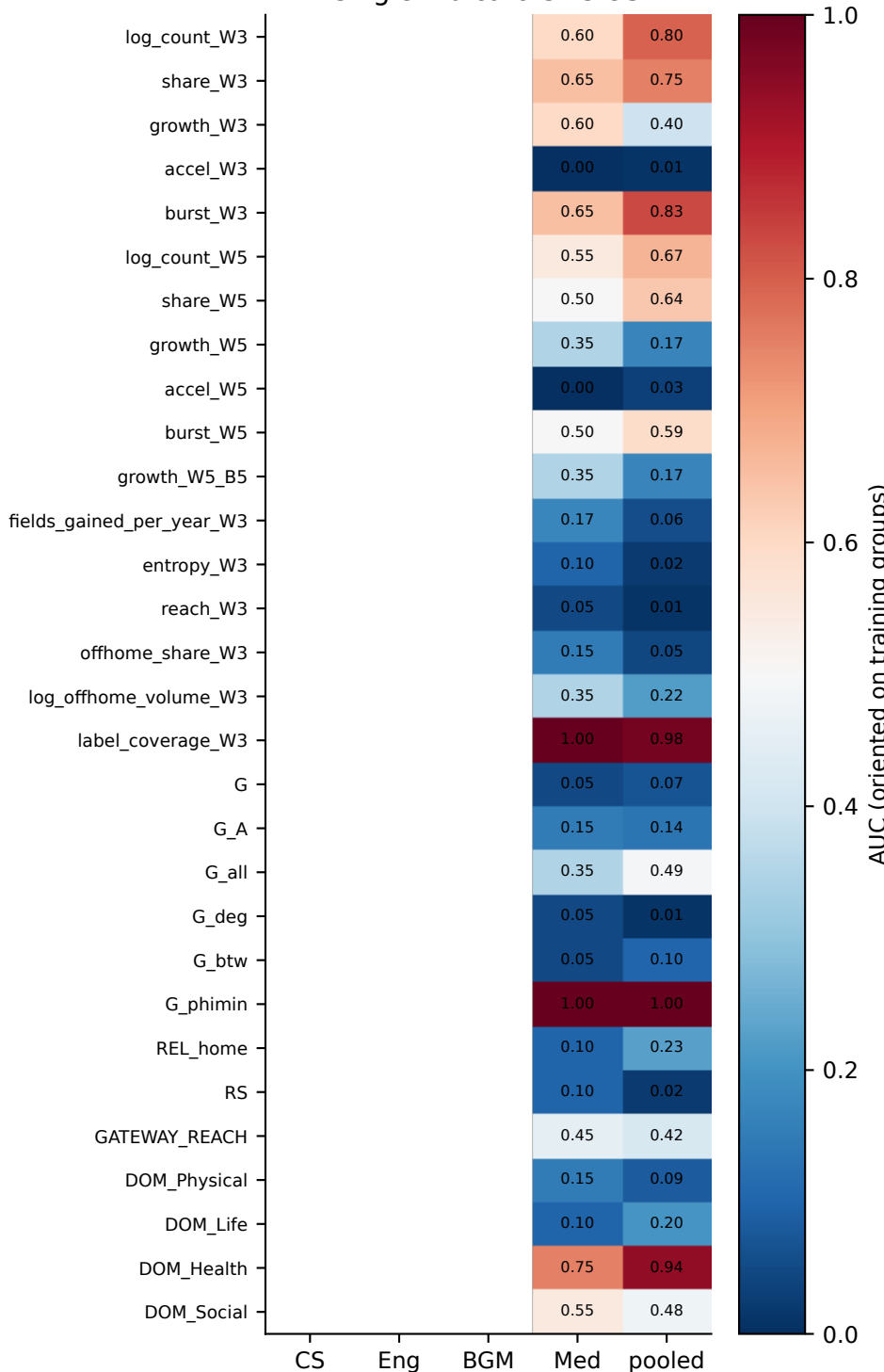
single indicators vs O3
