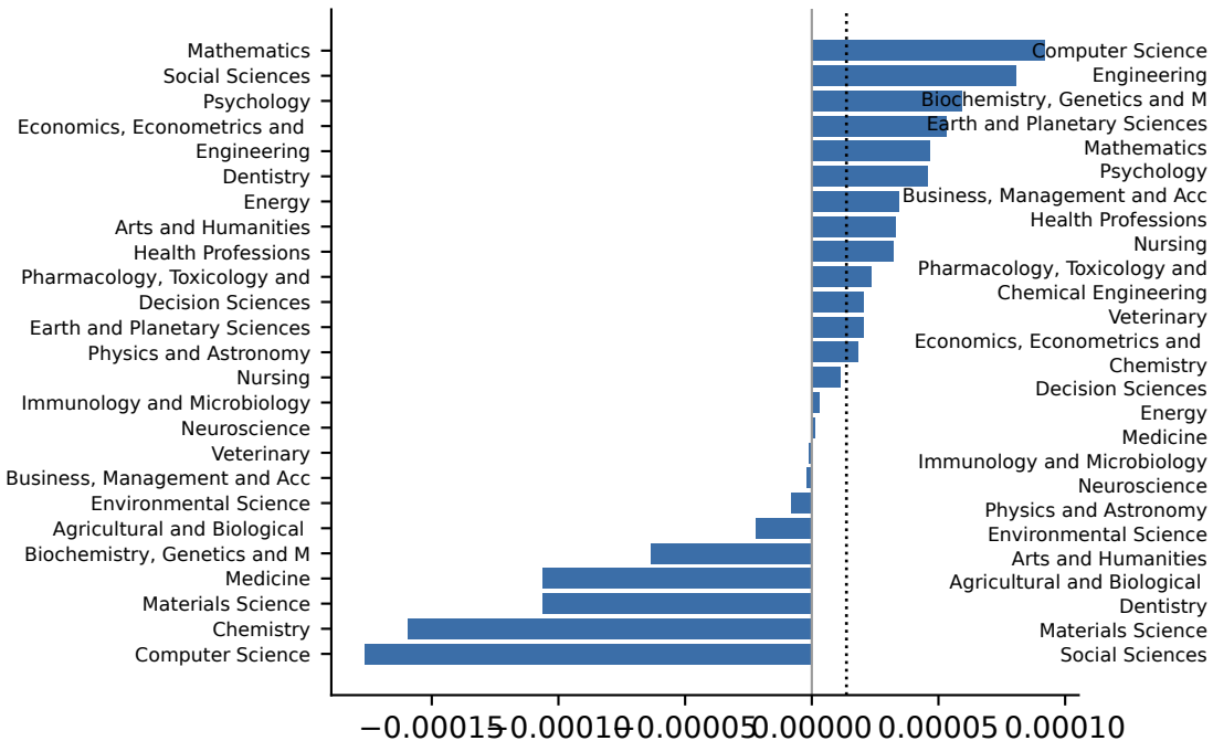
DEV: \Delta AUC leaving one adopting field out
