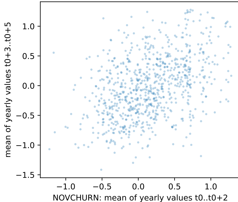
yearly windows, rho=0.41 (n=809)
