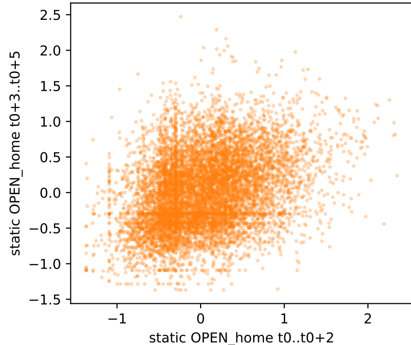
static 3-year build, rho=0.33 (n=9023)
