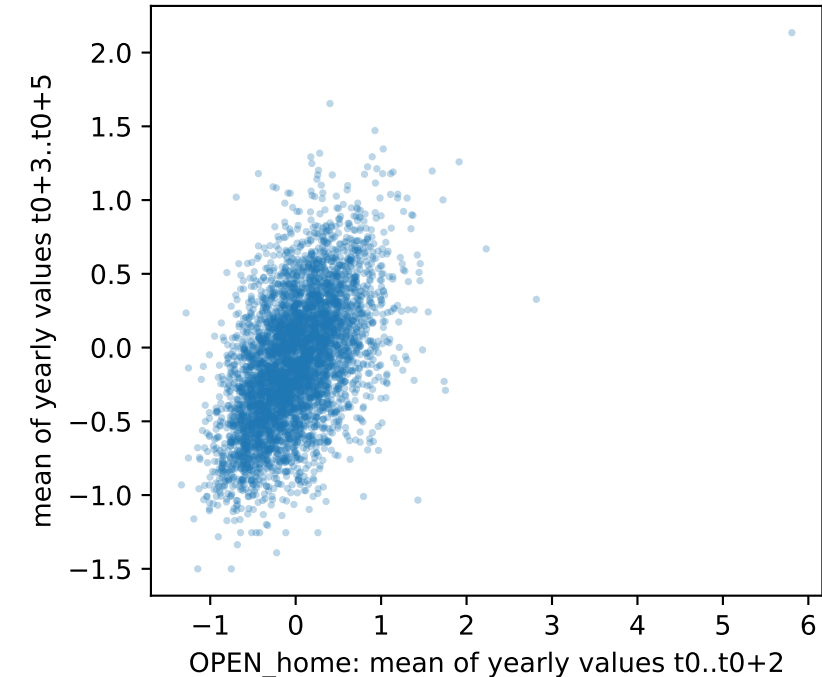
yearly windows, rho=0.54 (n=4607)
