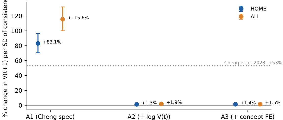
Test A: Cheng's volume effect of consistency, with and without current size
