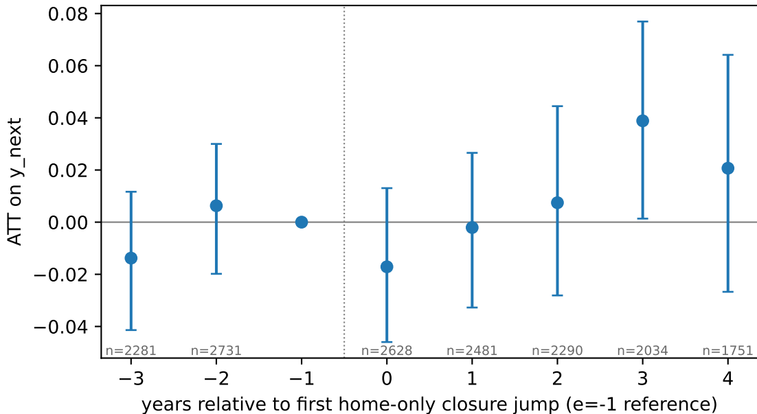
DEV - not_yet_treated_last_cohort (Sun-Abraham IW, 500 boots)
