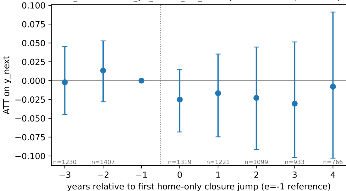
OLD_HELDOUT - not_yet_treated_last_cohort (Sun-Abraham IW, 300 boots)
