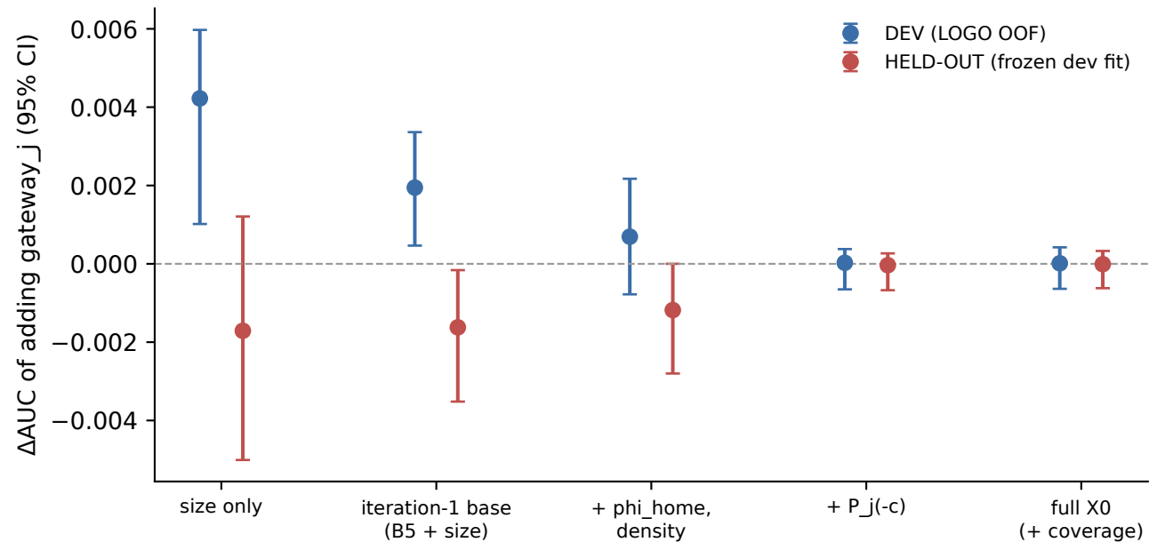
Gateway alone: AUC 0.605 (dev) vs 0.506 (held-out)
