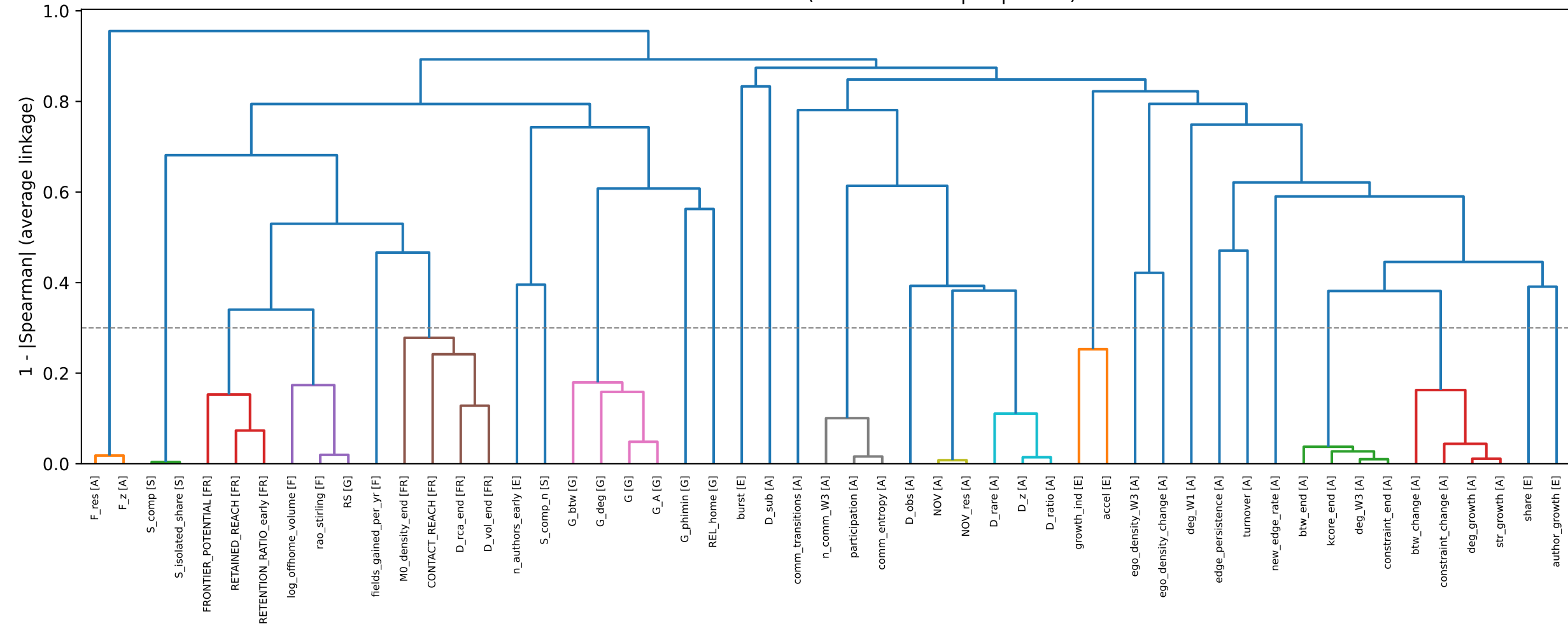
DEV indicator clusters (29 clusters at |\rho| < 0.7 )
