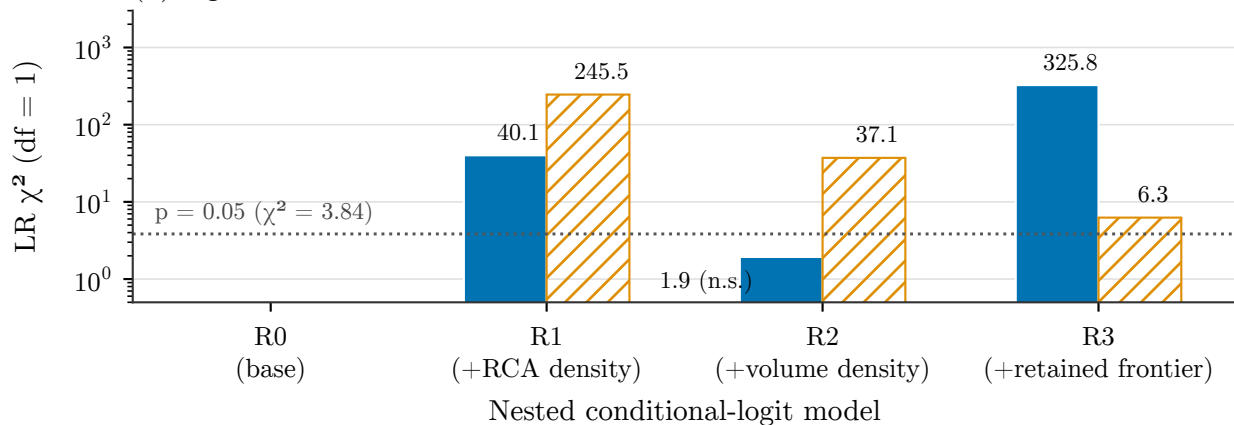
(b) Significance of each added term
