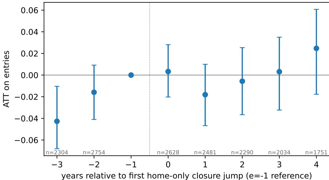
DEV - outcome_entries_t (Sun-Abraham IW, 300 boots)
