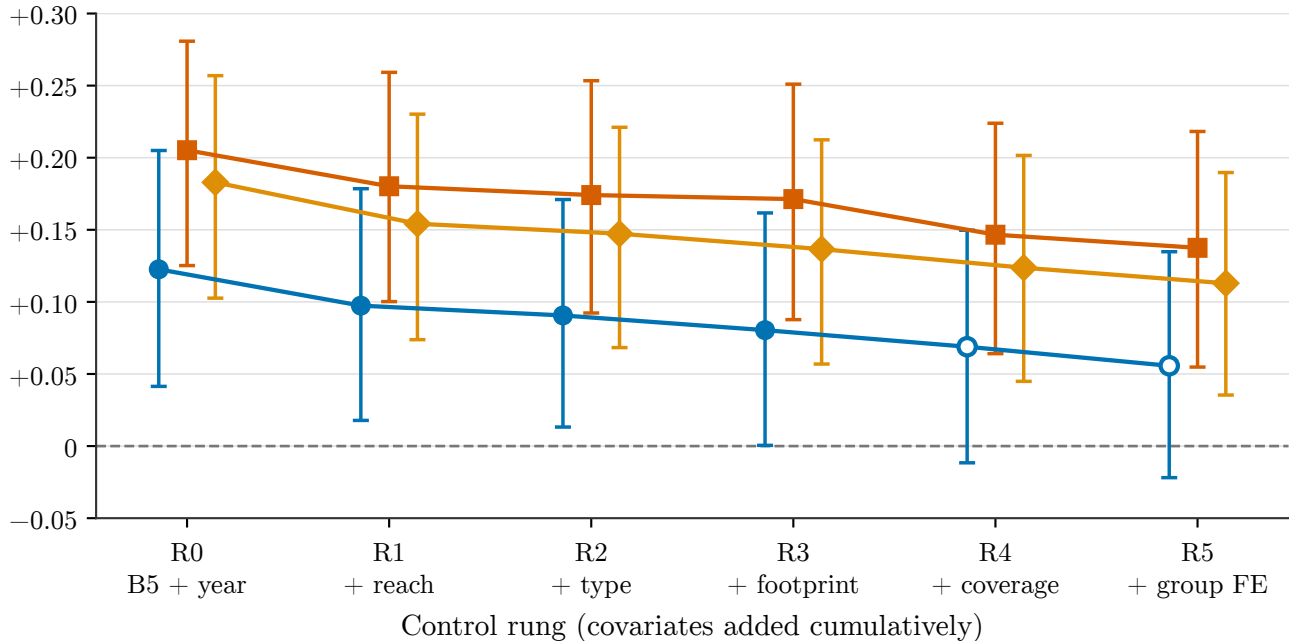
Partial Spearman \rho with later breadth
