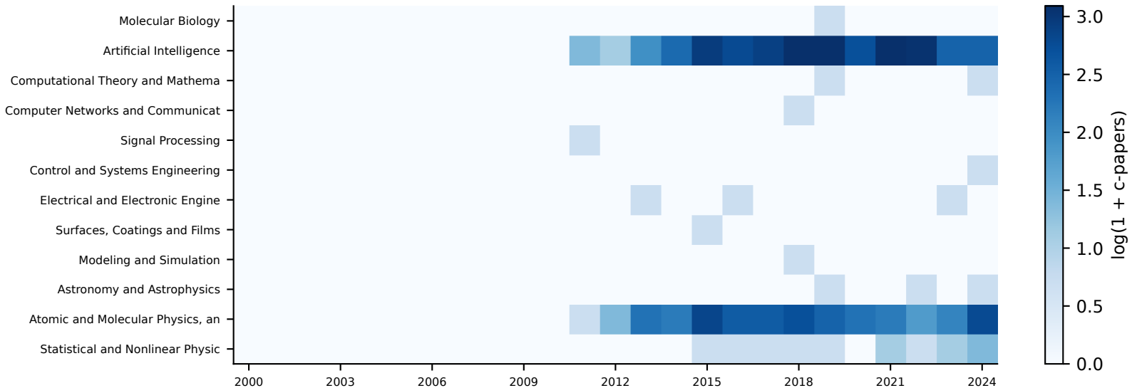
einstein podolsky rosen steering: c-papers by subfield and year
