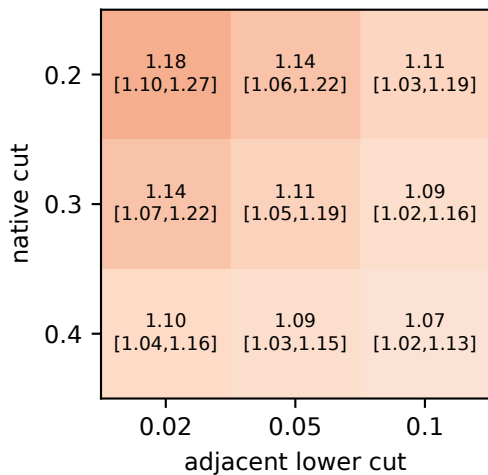
pooled: NATIVE share IRR/SD
