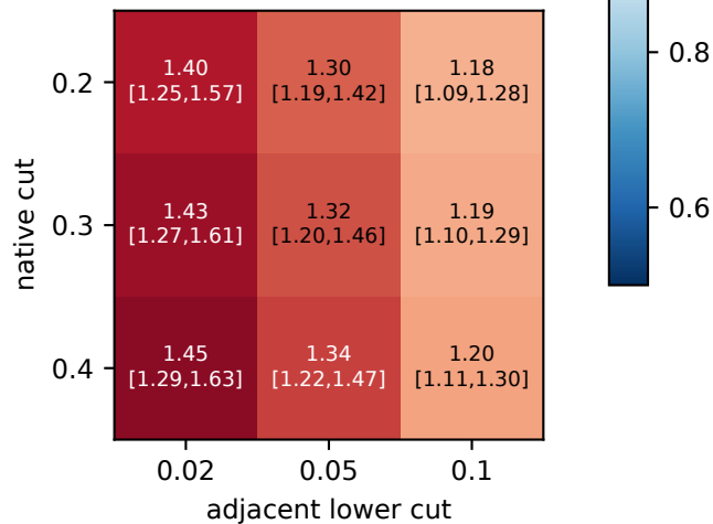
pooled: ADJACENT share IRR/SD
