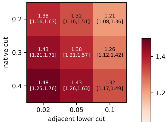
screen: ADJACENT share IRR/SD
