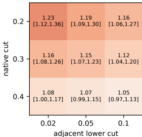
screen: NATIVE share IRR/SD
