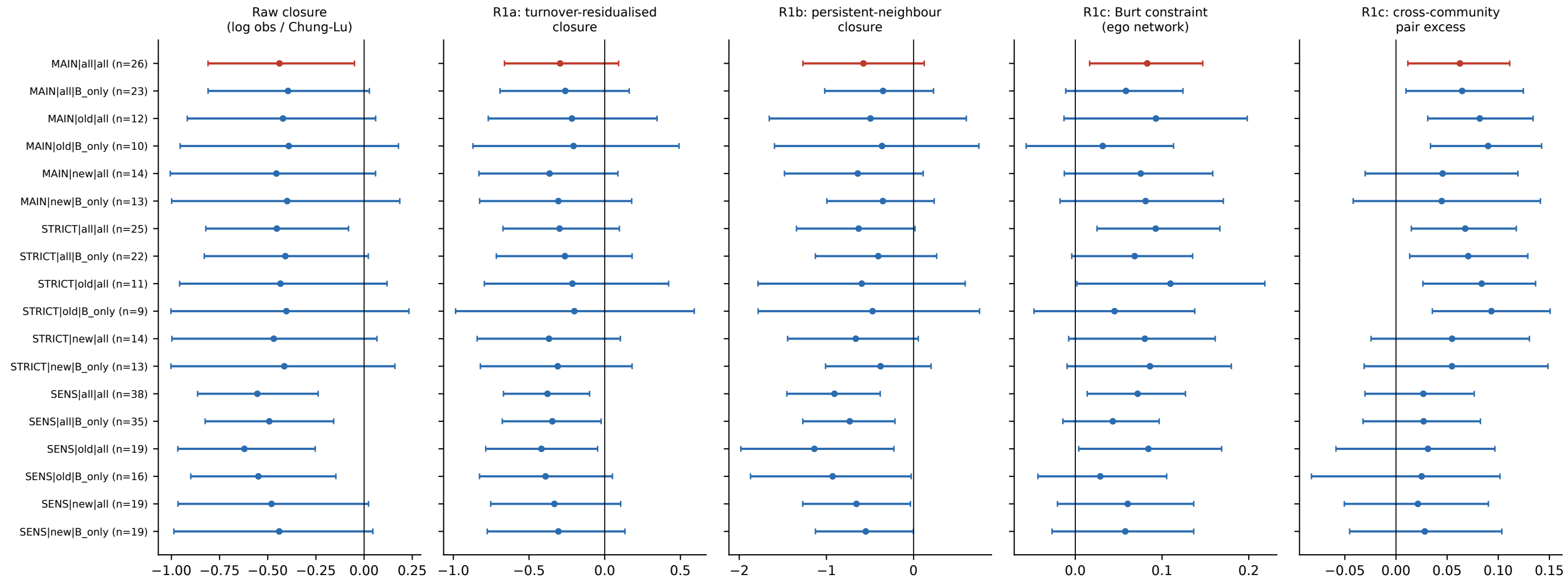
S ( k=-3.0 ) by population x subset x route, label E_up (primary cell in red; 95% CIs)
