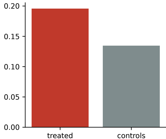
share d\_wmz > 0 & d\_closure < 0 ( k = -3..0 ) diff 0.061 [-0.009, 0.133]
