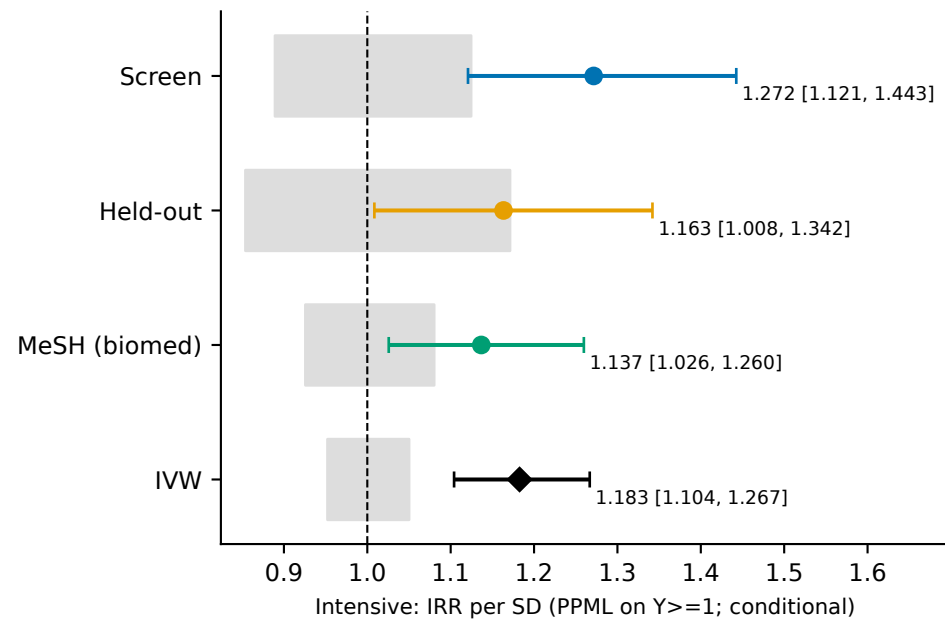
K1: which margin (post-confirmation exploratory; 95% CI, t(G-1) per fold, normal for IVW)
