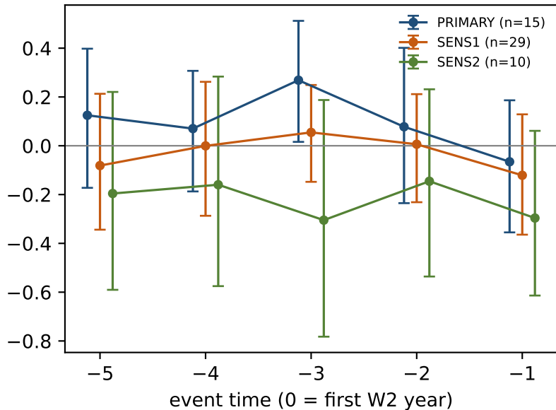
accretion_share
