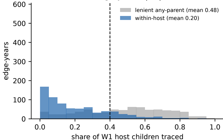
Main arm host edge-years, |Kd| \geq 10 (n=724)
