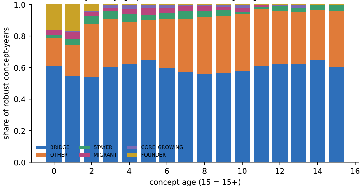
Community roles by age (pool-relative variant; roles agreeing in \geq 3/5 Leiden seeds)
