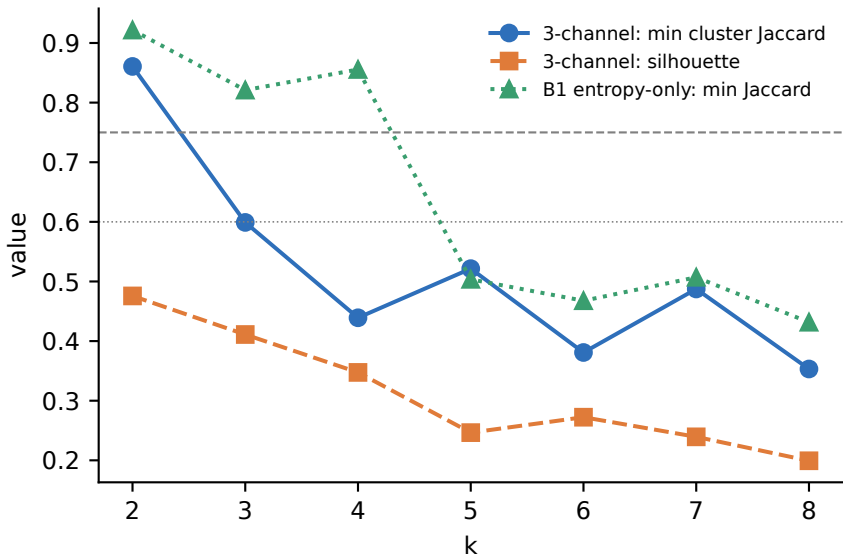
Hennig bootstrap stability (200 resamples)
