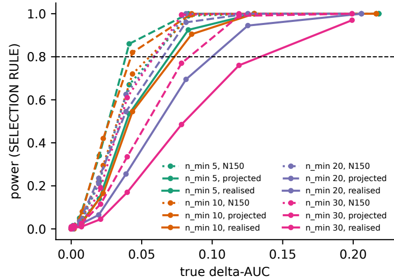
H1 power (delta-AUC), oracle BASE AUC 0.7
