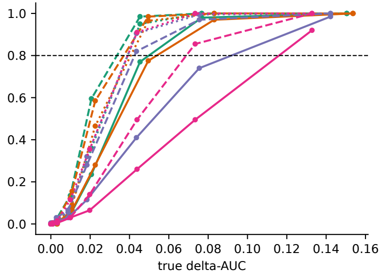
H1 power (delta-AUC), oracle BASE AUC 0.8
