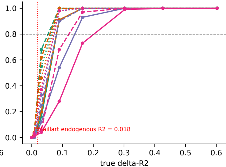
Continuous variant, BASE R2 0.10
