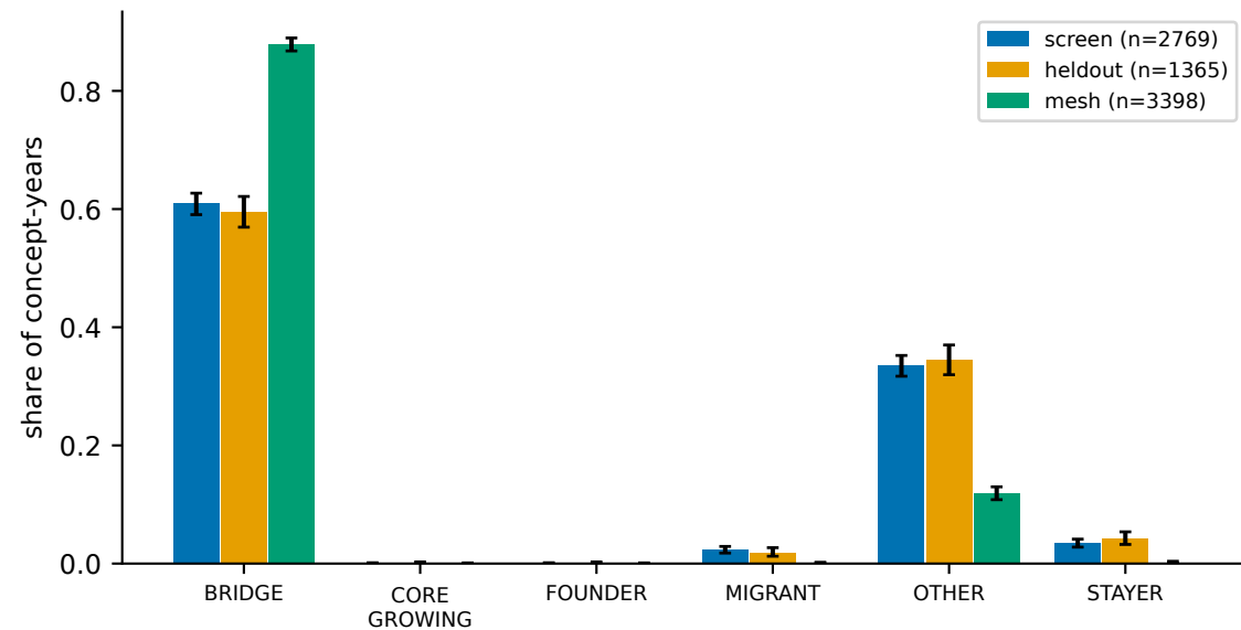
a. robust primary role shares
