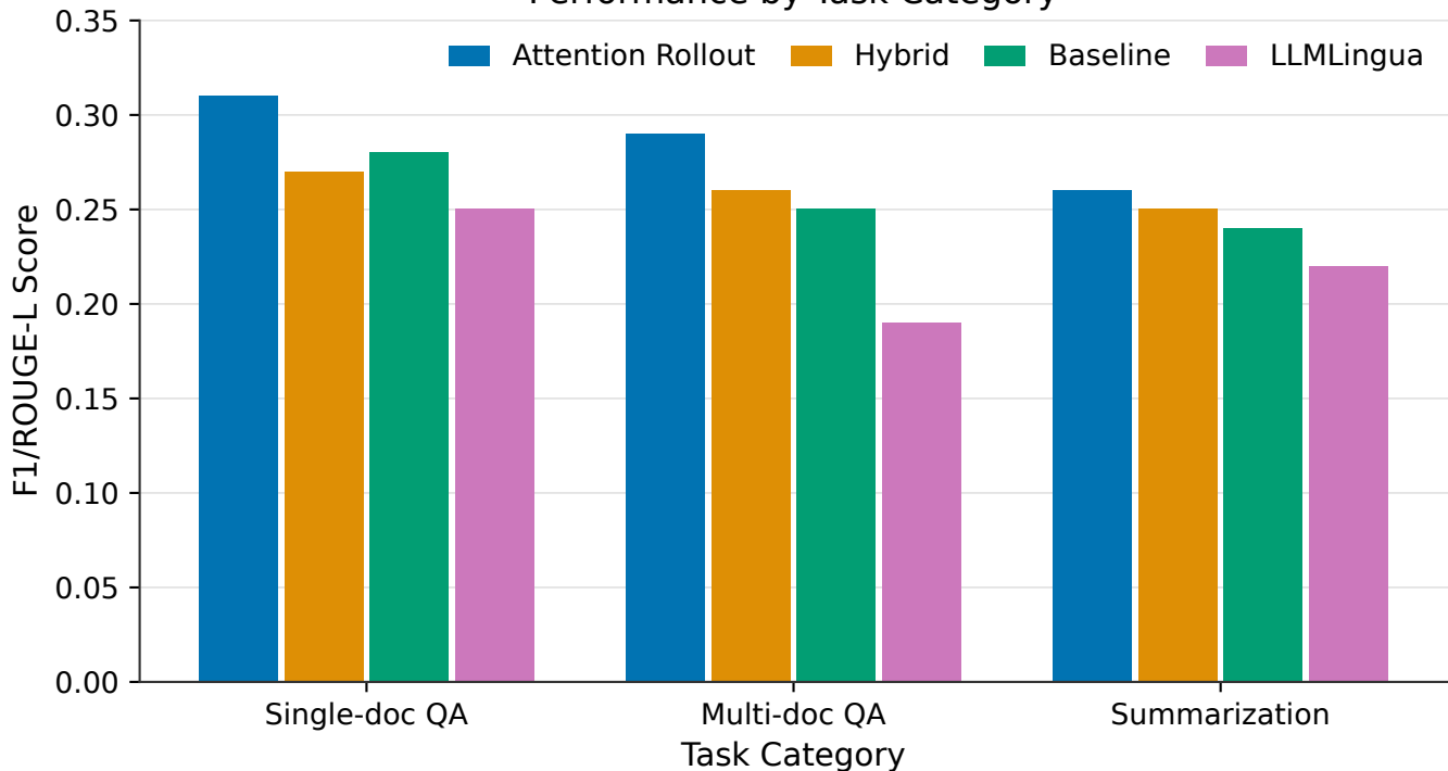
Performance by Task Category
