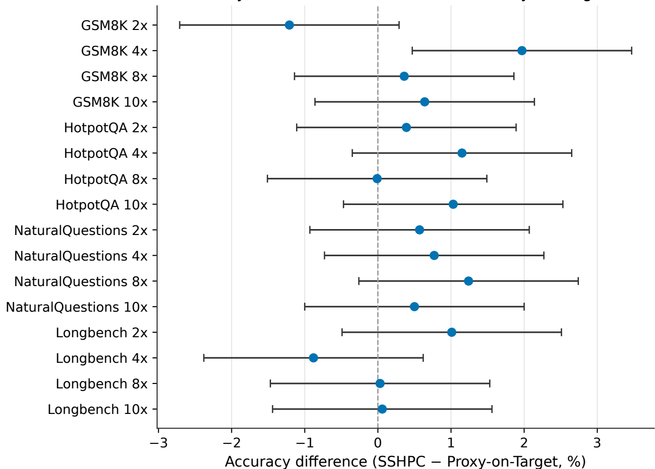
Proxy-Mismatch Ablation: SSHPC vs Proxy-on-Target
