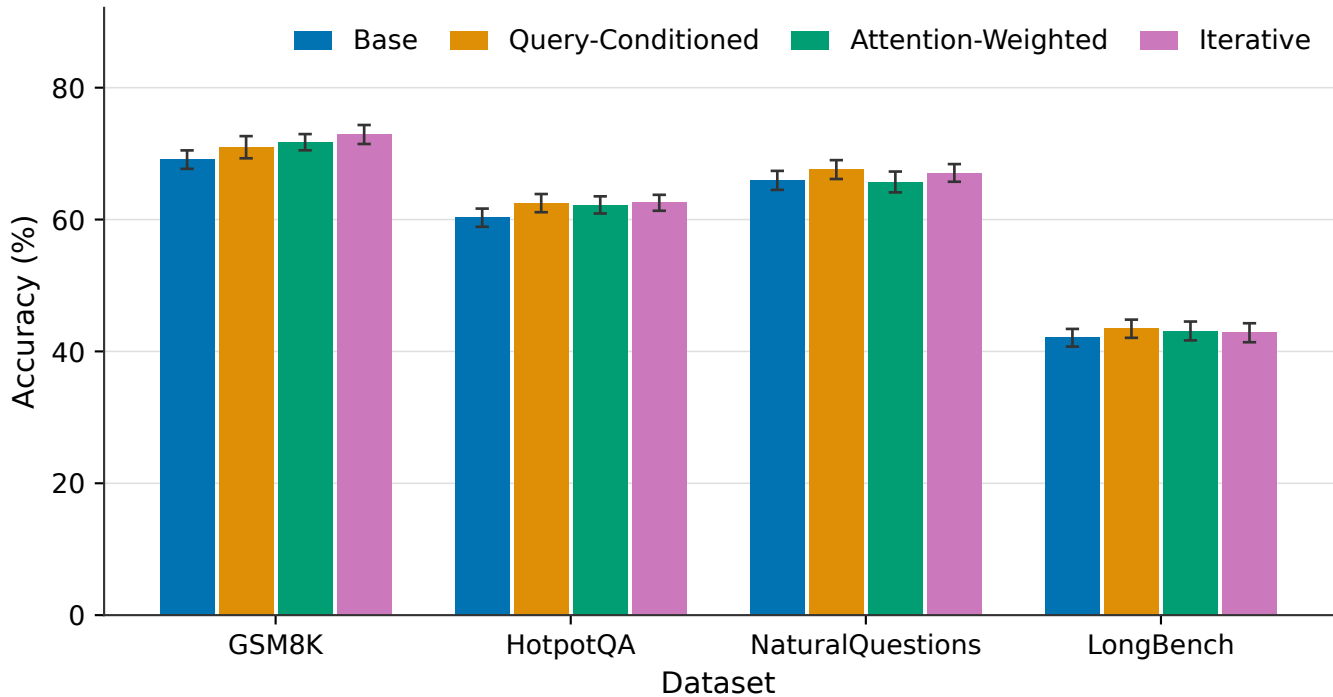
SSHPC Variant Comparison at 8x Compression
