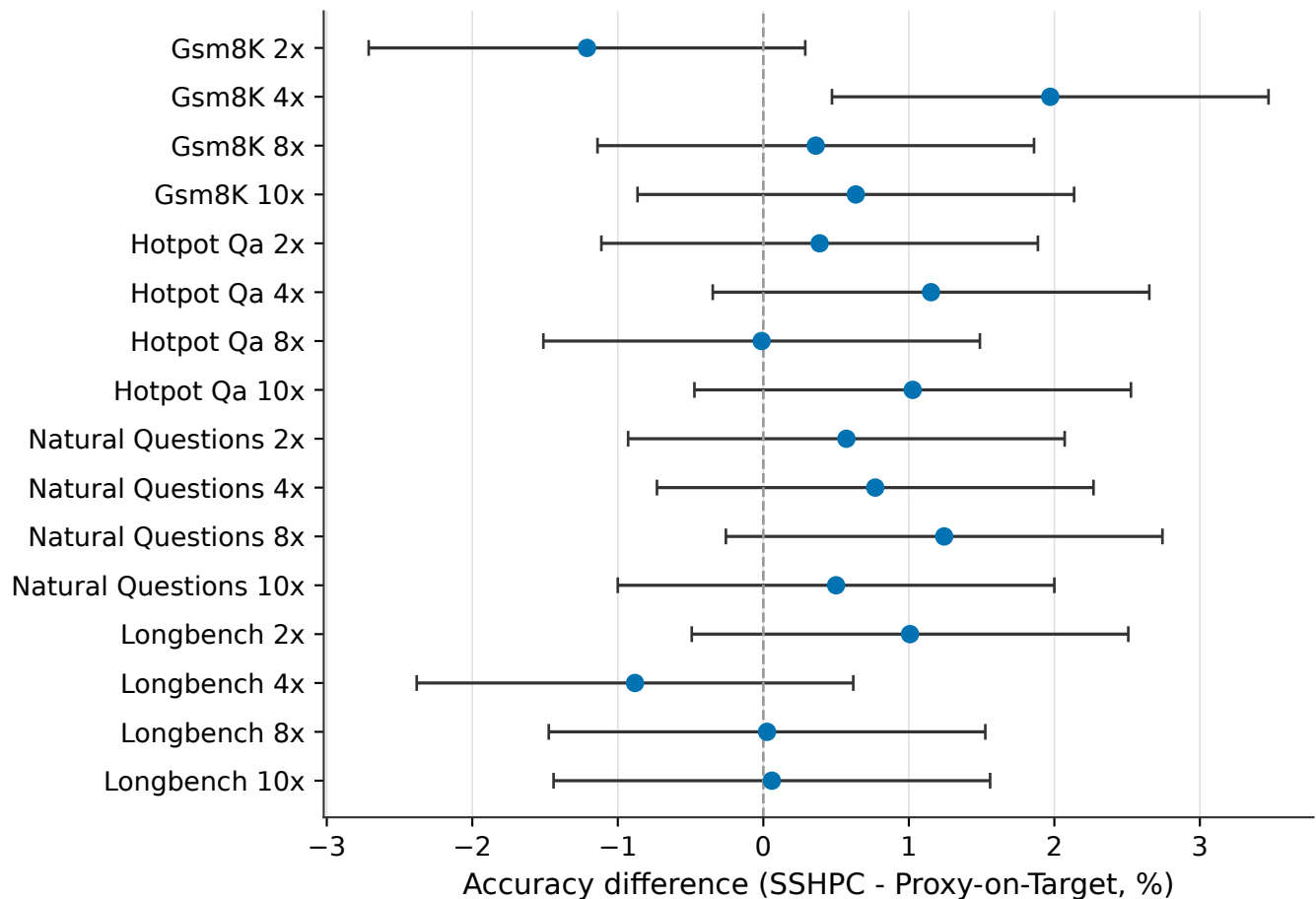
Proxy-mismatch effect: SSHPC vs Proxy-on-Target (same target LLM)
