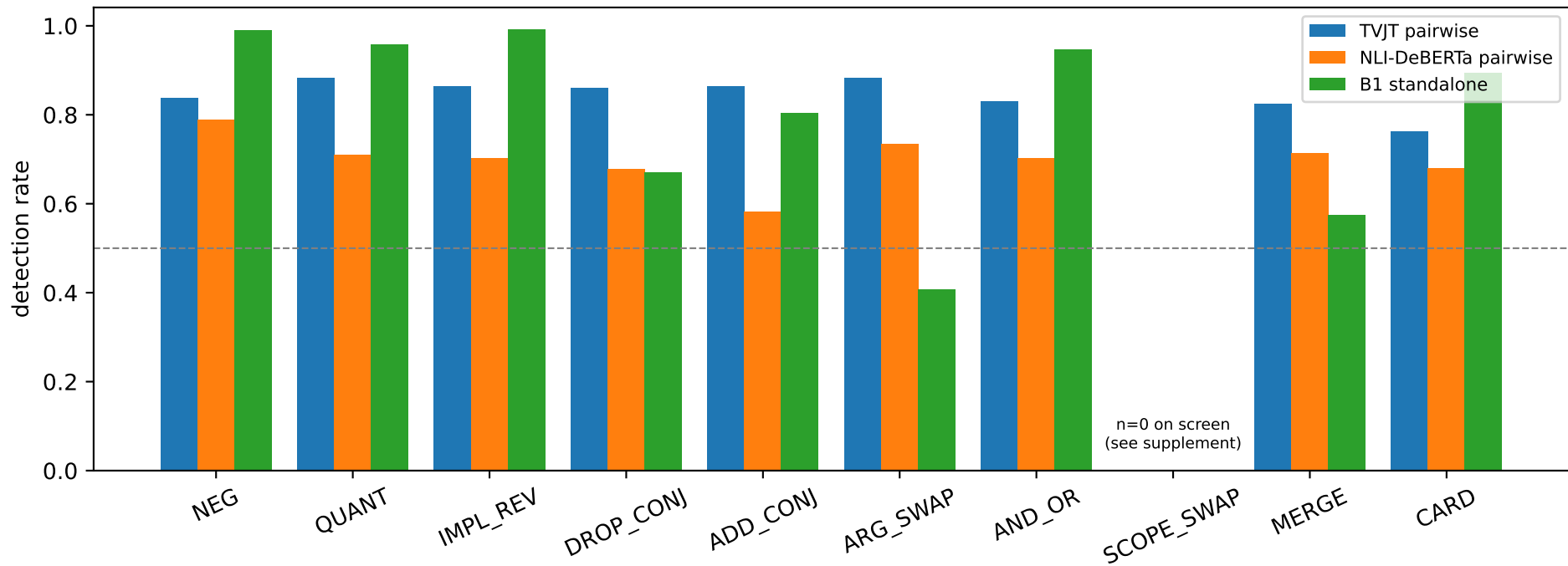
Per-operator detection on screen golds' controlled mutants (pairwise: judge sides with gold)
