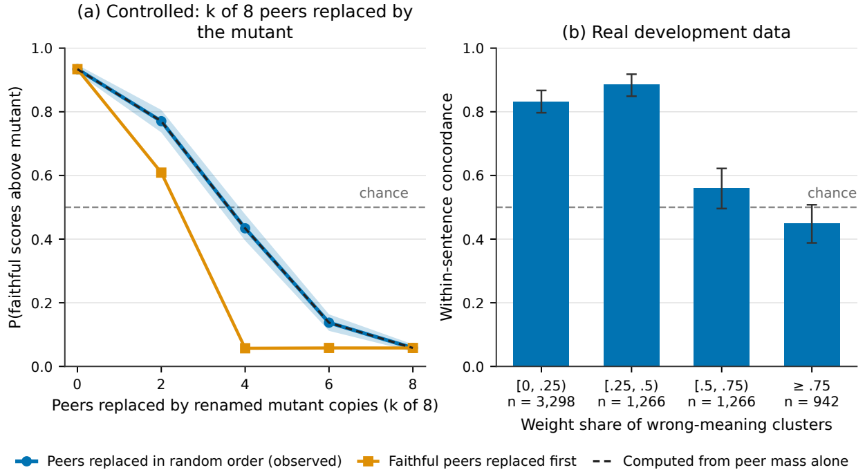
Figure 7: The shared-bias boundary of directional consensus on the development set. (a) Controlled shared error: probability that the faithful formula outscores a mutant as k of its 8 peers are replaced by renamed copies of the mutant (560 items from 200 sentences, four operators; 95% CIs for the random-order curve). The observed curve equals the curve computed from peer mass alone. (b) Real shared bias: within-sentence concordance over 6,772 faithful \times unfaithful pairs, binned by the weight share of wrong-meaning clusters in the sentence (logistic slope -2.08 [ -2.55, -1.61 ]).
