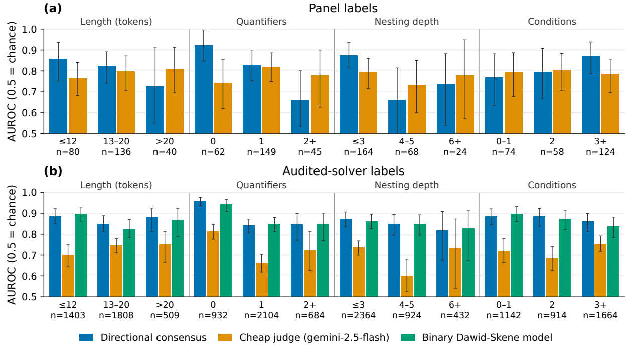
Figure 9: Fresh confirmation set: AUROC of directional consensus and the cheap judge in each complexity stratum the user named. (a) Panel labels (n items per stratum in the category labels). (b) Audited-solver labels, with the binary Dawid-Skene model added. Under panel labels agreement leads on short, quantifier-free and shallow items and trails the judge on sentences with two or more quantifiers, nesting depth 4-5 and more than 20 tokens; it also leads on sentences with three or more conditions (0.871 against 0.787). The tercile gap to the judge shrinks (+0.088, +0.107, -0.028; slope -0.058 [-0.135, 0.022], not significant). Solver labels share DC’s equivalence checker, so panel (b) is partly circular.
