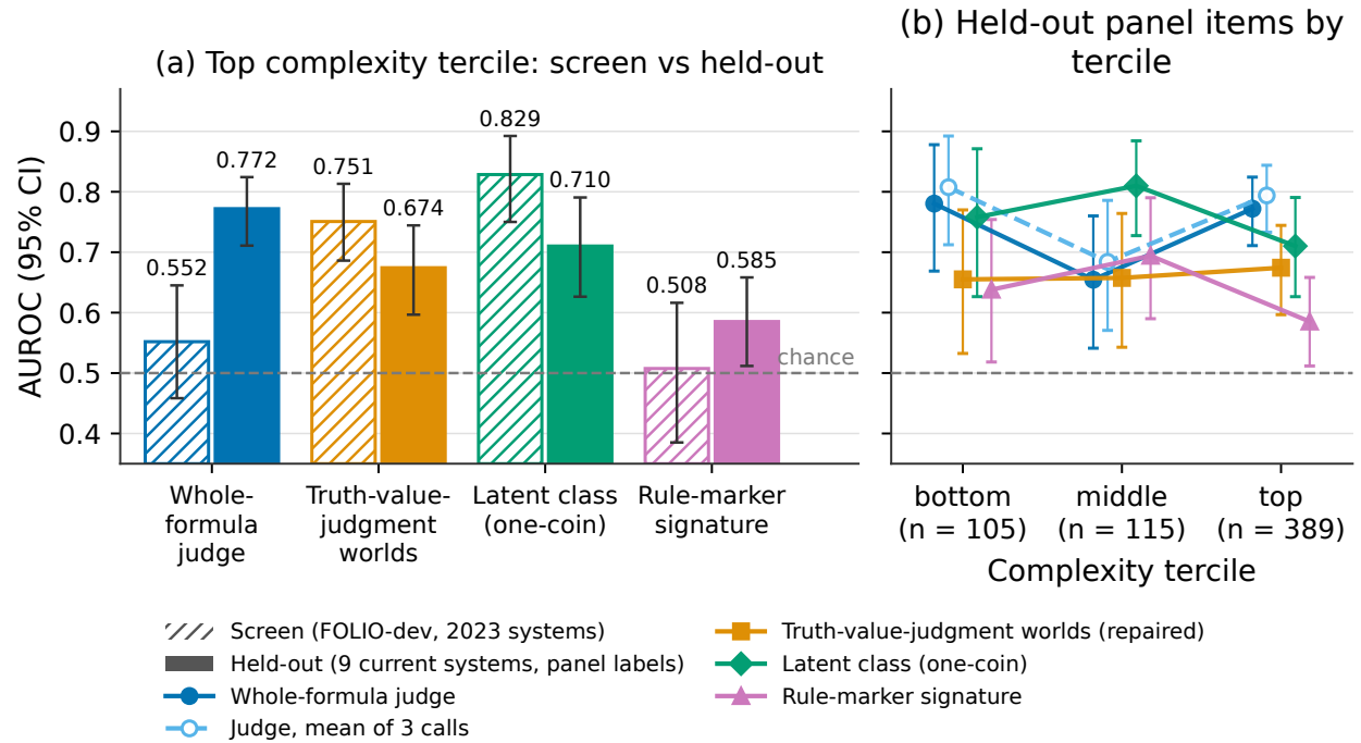
Figure 5: Panel (a): AUROC in the top complexity tercile on the iteration-1 FOLIO-dev screen (Logic-LM candidates; worlds, latent class and judge against Arm B labels, n = 833 overall; rule-marker signature against Arm A labels) and on the held-out panel items (389 top-tercile items, post-stratified weights; truth-value-judgment worlds in their repaired, frozen form). Panel (b): held-out panel AUROC by tercile (bottom n = 105 , middle n = 115 , top n = 389 ). The judge fell to 0.552 on the screen’s top tercile but scores 0.772 on held-out top-tercile items, where the worlds are 0.098 below it.
