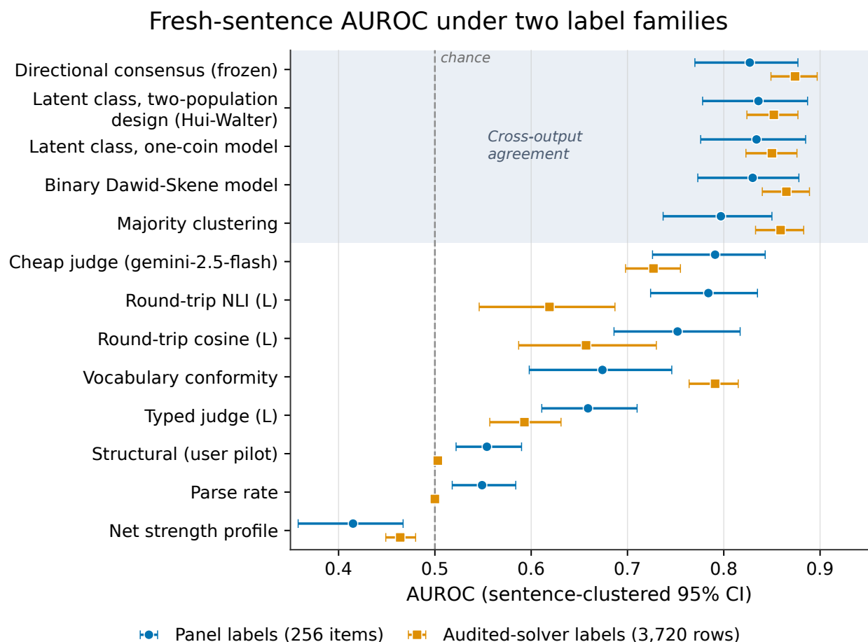
Figure 8: Fresh confirmation set (450 new sentences \times 9 systems): AUROC with sentence-clustered 95% CIs under panel labels (256 adjudicated items, raked weights) and audited-solver labels (3,720 rows; 260 rows for the local round-trip and typed-judge substitutes, marked L). Cross-output agreement (directional consensus and the latent-class variants) leads under both labels; the cheap judge drops from 0.791 to 0.727 when the labels switch to solver equivalence; parse rate and the user’s structural metrics sit at chance; the directional strength profile ranks below chance.
