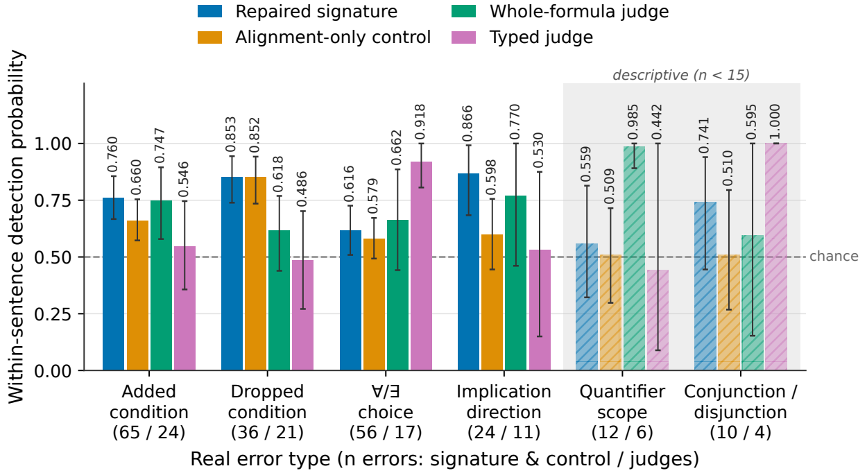
Figure 6: Within-sentence detection by real (panel-typed) error type on held-out data: probability that an erroneous candidate scores below a faithful candidate of the same sentence ( 0.5 = \text{chance} ). The signature and alignment-only control were scored on every item with a partner; the judges only on the items they covered ( n in the category labels). The repaired signature leads on dropped conditions and implication-direction errors and trails the typed judge on the \forall/\exists choice. Post hoc: the two leading classes were singled out from nine after the data were seen, the judges were scored only on the items they happened to cover, and with the cheap judge re-scored on all available pairs it detects dropped-condition and implication-direction errors at 0.577 and 0.576 (Table 37).
