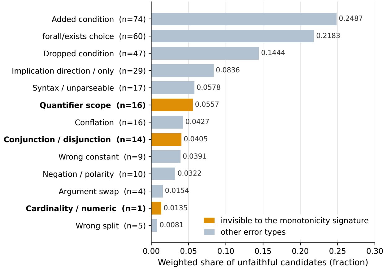
Figure 3: Primary error type among held-out candidates the three-model panel judged unfaithful, post-stratified weighted shares (609 adjudicated greedy candidates from 9 current systems on MALLS, FOLIO-v2-train and ProverQA). Error types the monotonicity signature cannot see (quantifier scope, cardinality, conjunction/disjunction) are highlighted; scope plus cardinality is 6.9%.
