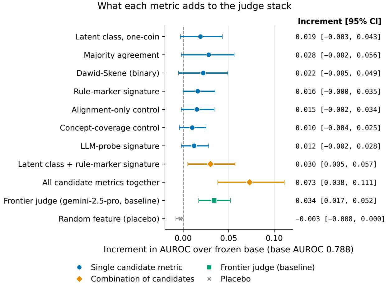
Figure 4: Held-out confirmation (609 panel-adjudicated candidates, post-stratified weights): increment in cross-fitted AUROC when each metric is added to the frozen base [whole-formula judge, parse rate, round-trip NLI, round-trip cosine, structural metrics] (base AUROC 0.788), with sentence-clustered 95% CIs. Only the frontier judge, a baseline, and combinations of candidates have a lower bound above zero; no single candidate metric does.
