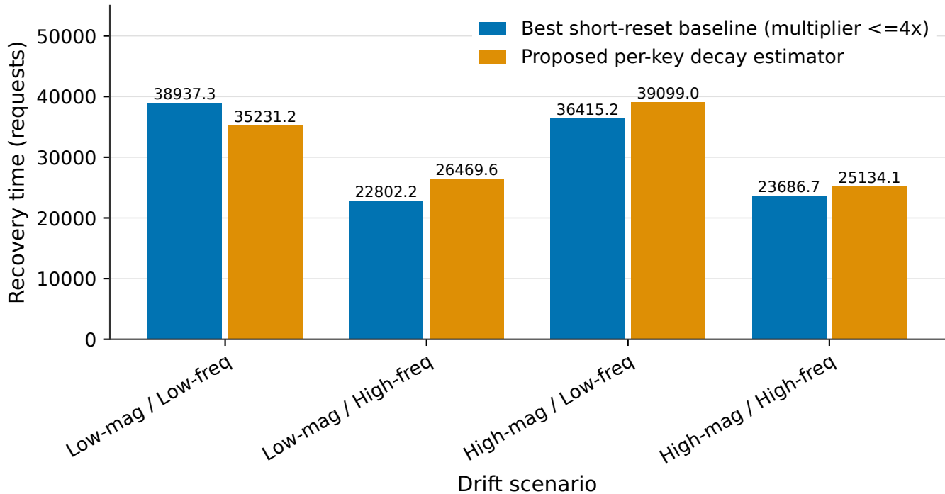
Short Reset vs Per-Key Decay
