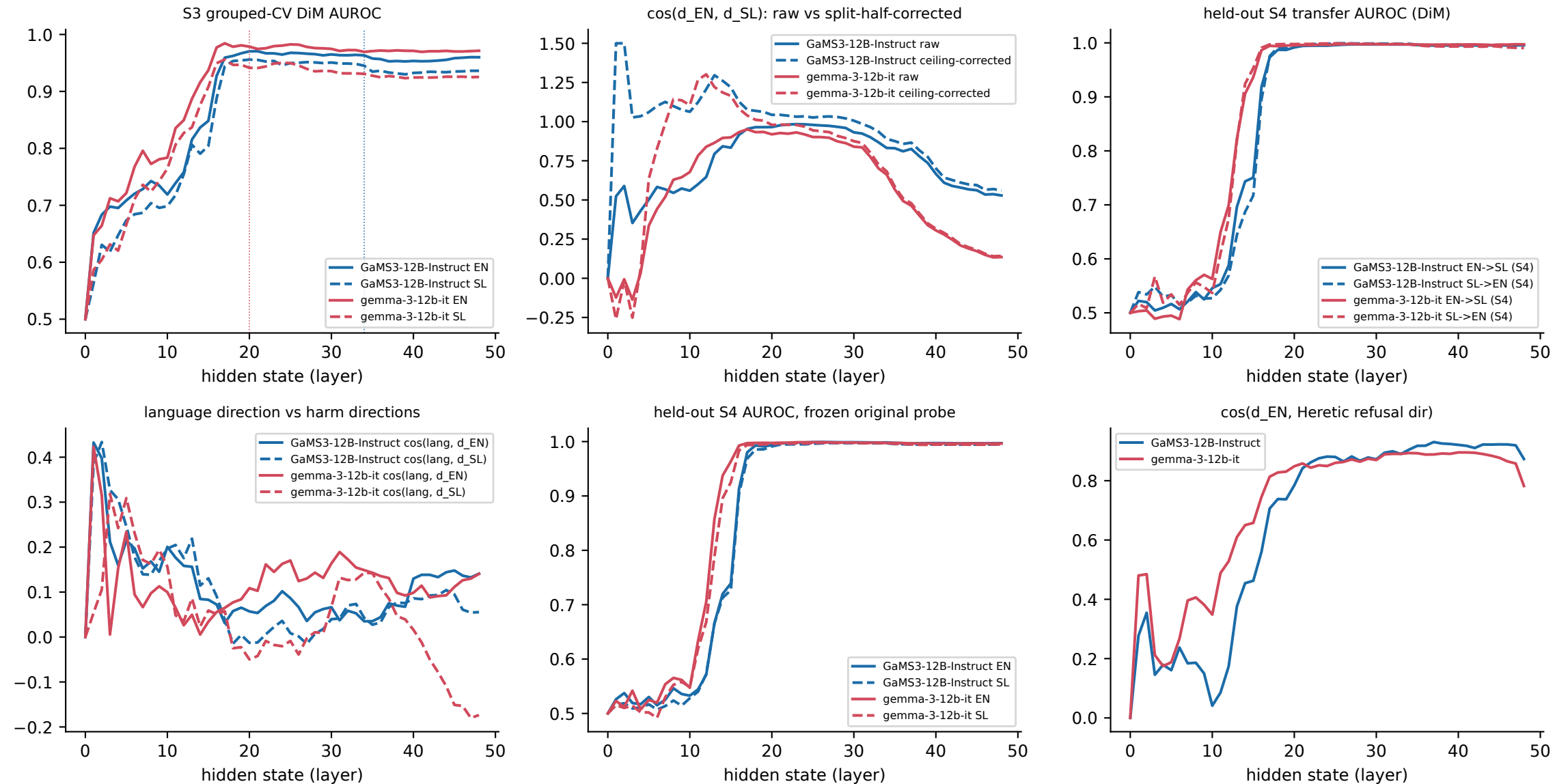
Fig. 2 Layer profiles (pos -1, winsorized float32; original models)
