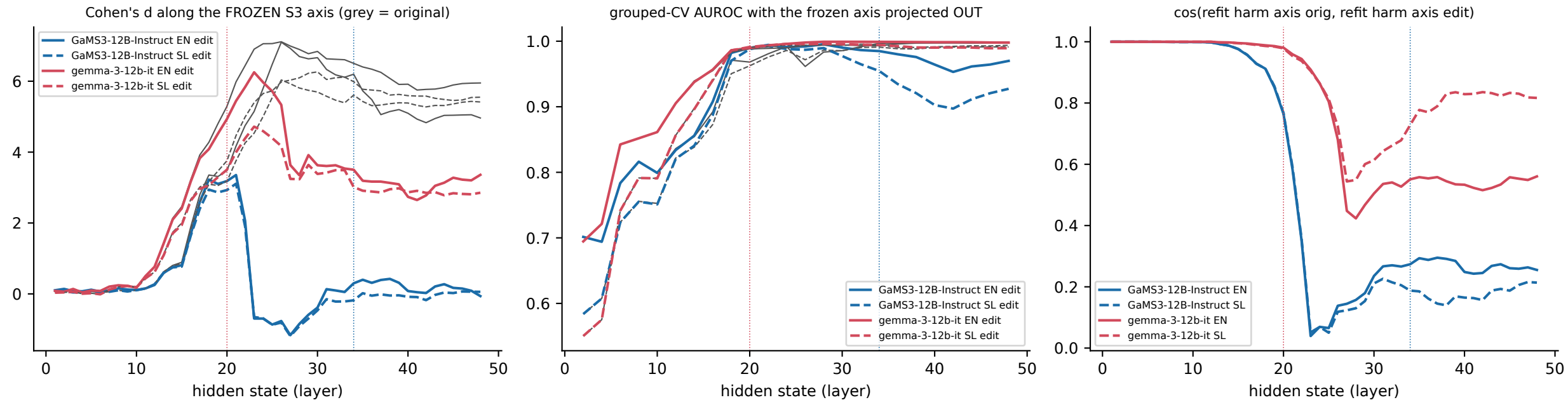
Fig. 7 Where the frozen probe fails: axis-aligned separation removed, off-axis information kept (S4, pos -1)
