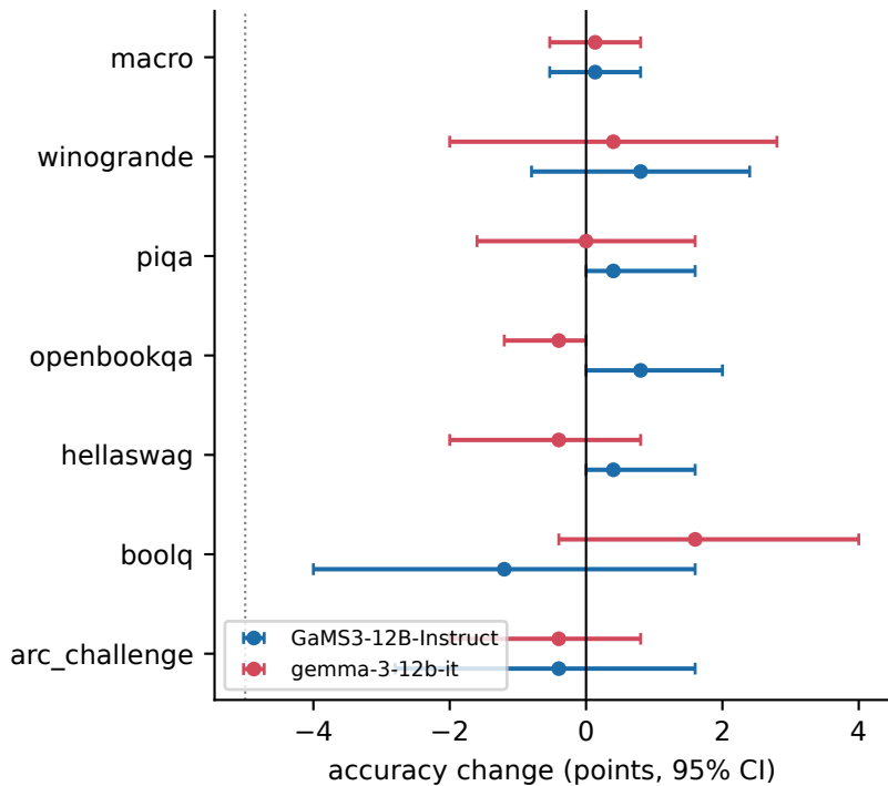
Fig. 1 Utility change after the Heretic edit (250 items/task, 0-shot, NF4)
