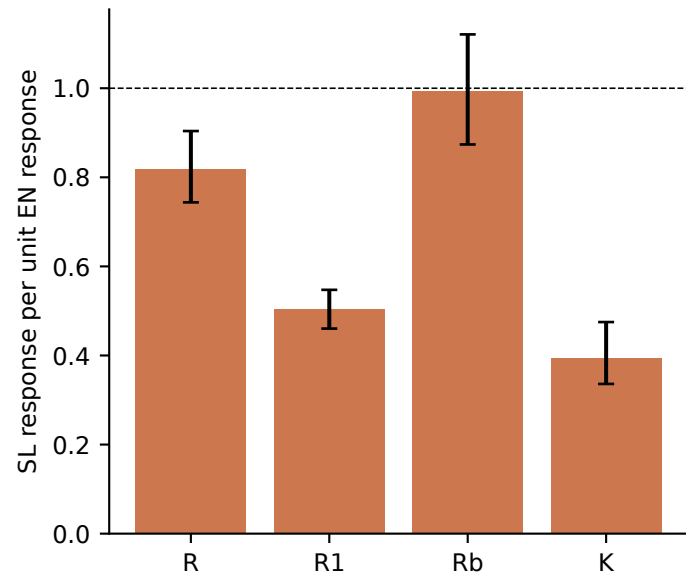
transfer ratio (exploratory; 1 = equal)
