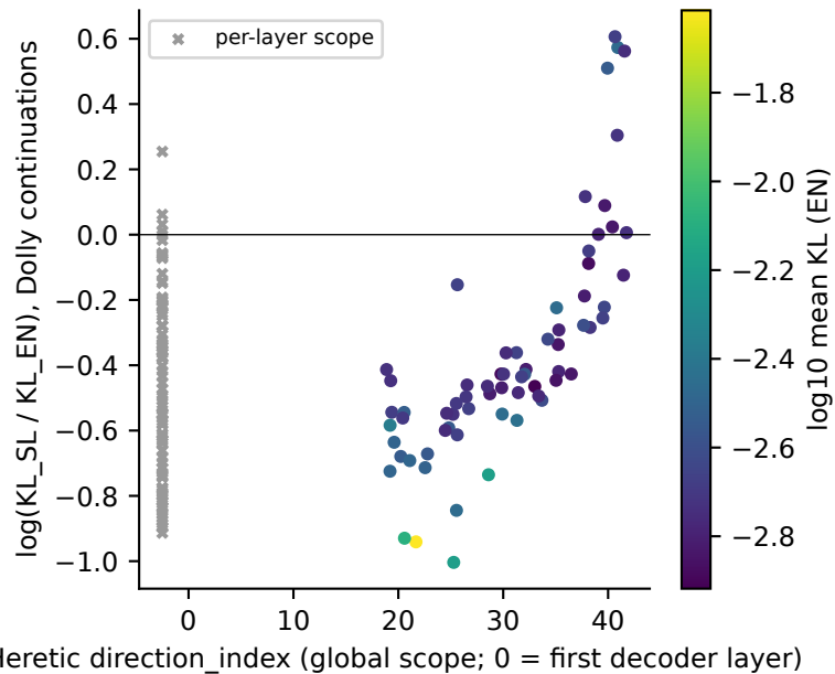
SL/EN divergence ratio vs refusal-direction layer (F)
