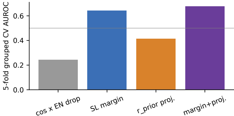
Which SL items survive d_EN?
