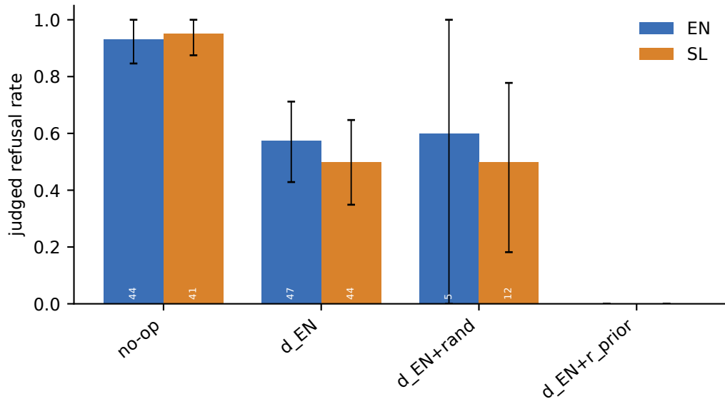
GaMS3-12B-Instruct, OUTCOME harmful
