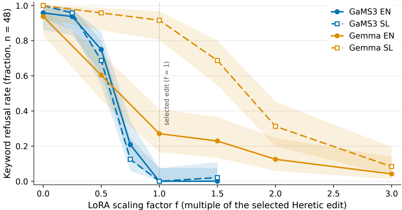
Keyword refusal vs. edit strength
