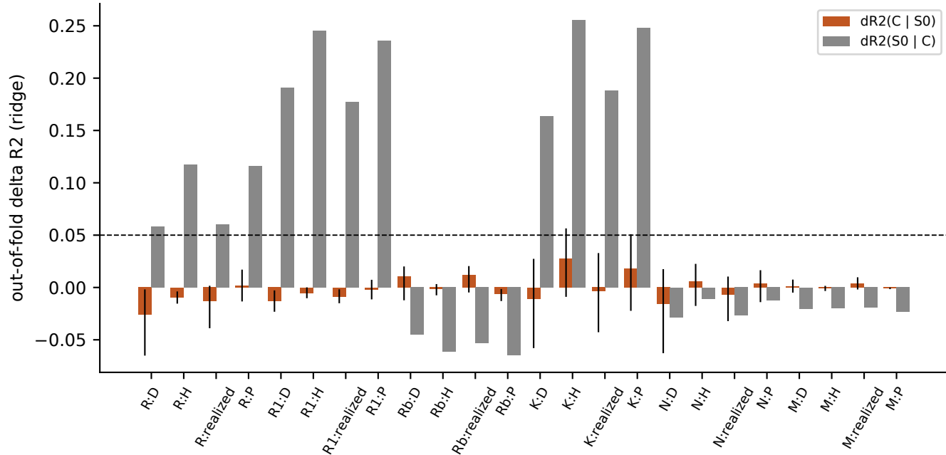
Carrier regression on the SL-minus-EN residual (S0 = cosine b1/b1x, lang b2, kernel mass b3, Omega)
