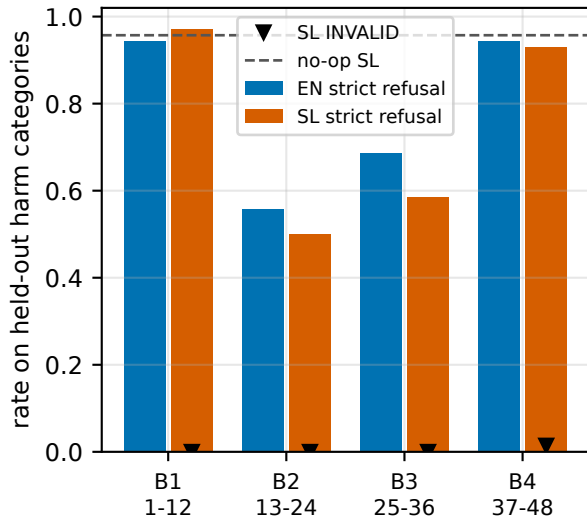
Where the same edit energy is placed decides what it removes matched energy E2
