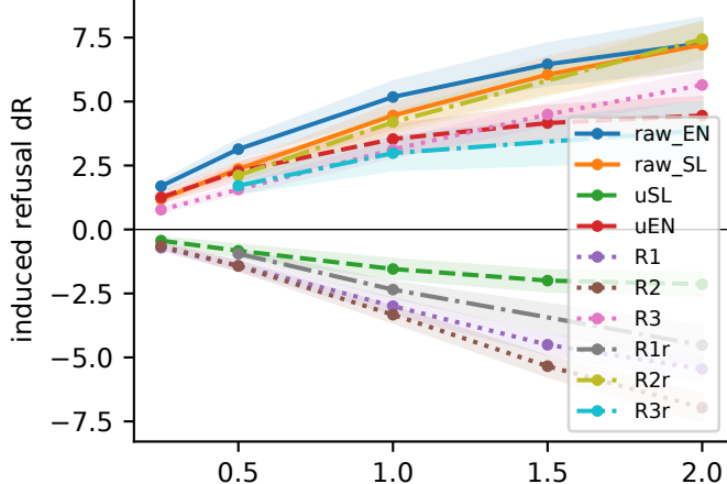
Gemma-3-12B-it: addition, benign twins, eval SL
