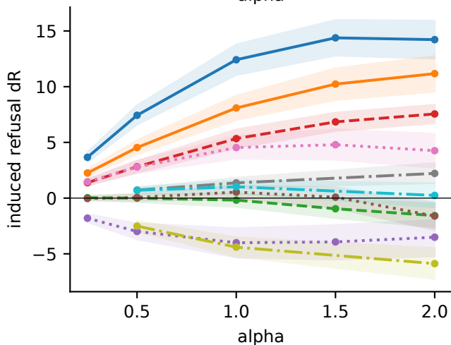
Gemma-3-12B-it: addition, benign twins, eval SL
