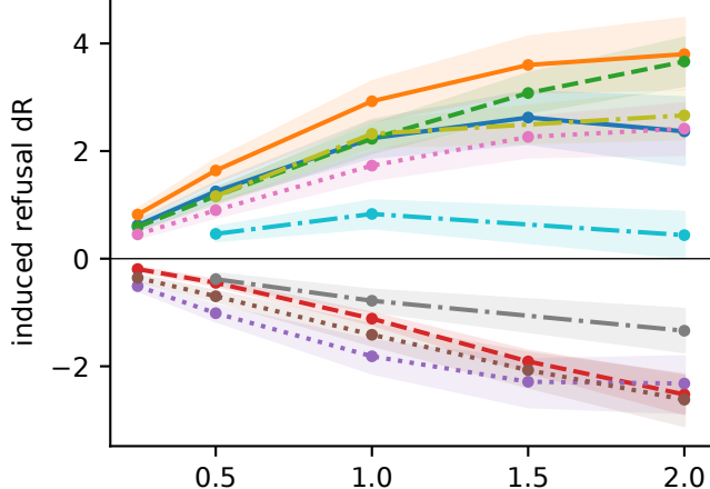
Gemma-3-12B-it: addition, benign twins, eval SL
